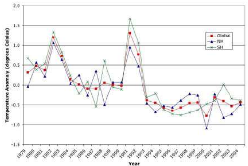
Winter MSU Stratospheric Temperatures
