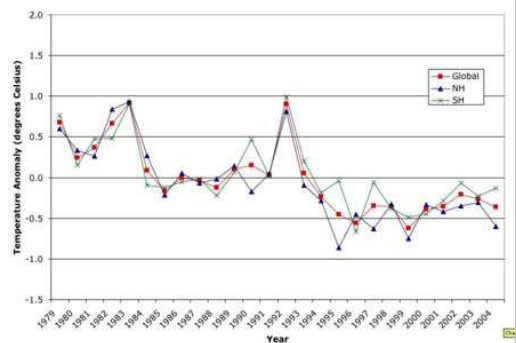
Spring MSU Stratospheric Temperatures
