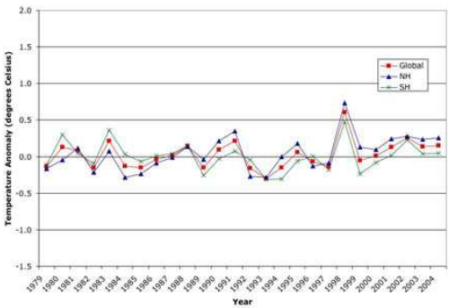
Summer MSU Tropospheric Temperatures
