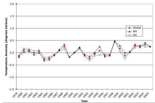
Winter MSU Tropospheric Temperatures
