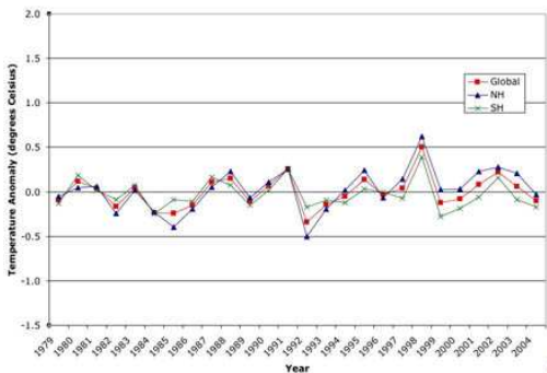
Summer MSU Tropospheric Temperatures
