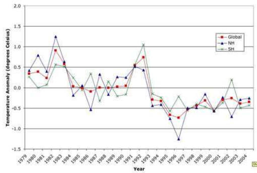
Autumn MSU Stratospheric Temperatures
