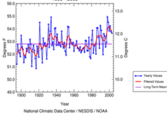
National (Contiguous U.S.) Temperature 1895 - 2003
