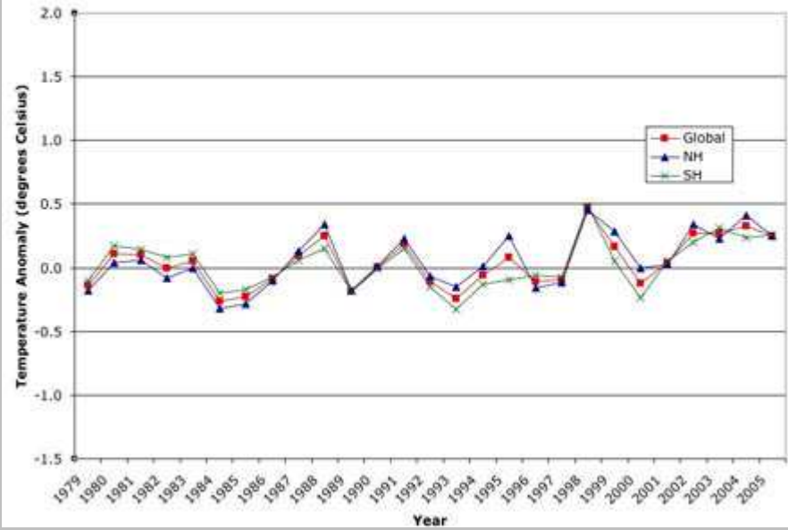
Winter MSU Tropospheric Temperatures
