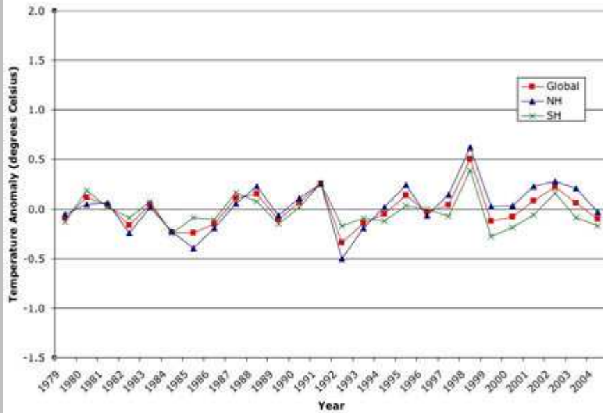
Summer MSU Tropospheric Temperatures
