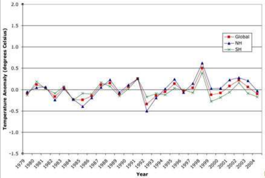
Summer MSU Tropospheric Temperatures
