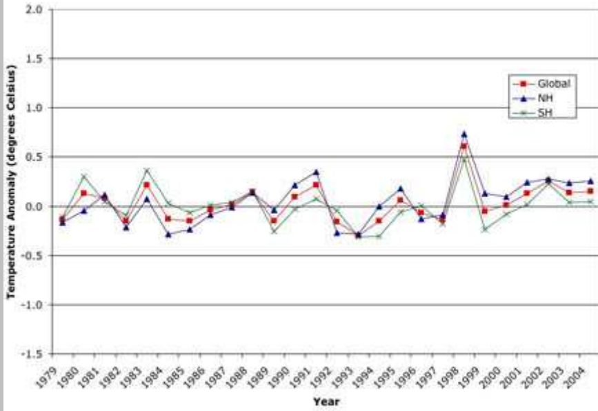
Spring MSU Tropospheric Temperatures
